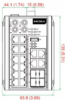
Front Views
