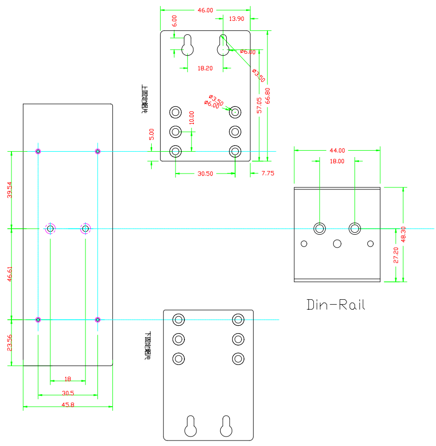
Panel Mount Kit
