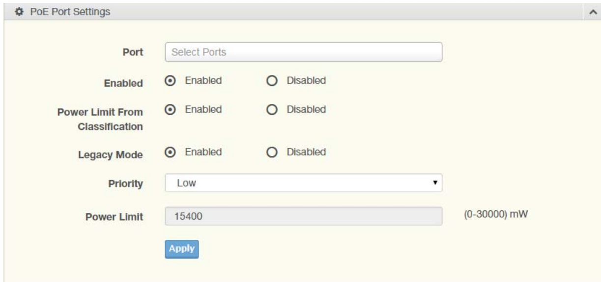
Figure 4.90 Management > Power Over Ethernet > PoE Port Settings
