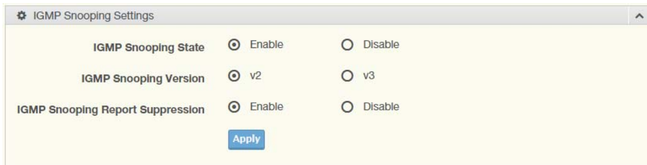
Figure 4.31 L2 Switching > Multicast > IGMP Snooping > IGMP Settings
