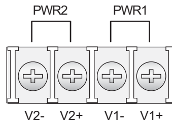
Figure 2.14 Terminal Receptor: Relay Contact
