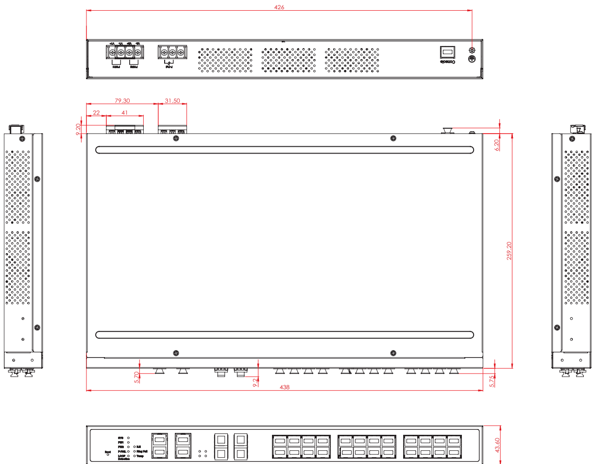
Figure 1.5 EKI-7428G-4CI Dimensions
